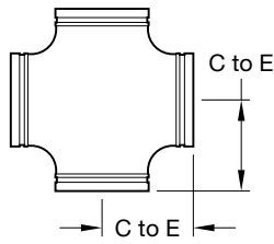
FIGURE 227 CAST CROSS
