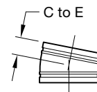
FIGURE 211 CAST 11-1/4° ELBOW
